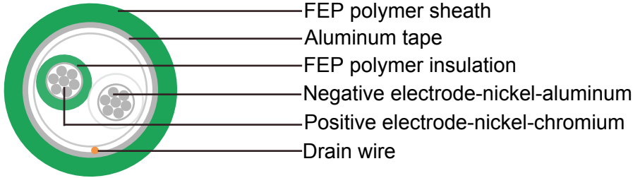
KX FEP insulated
